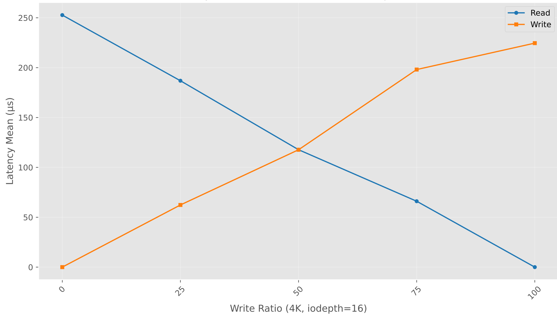
Latency Mean vs Write Ratio (4K, iodepth=16)
